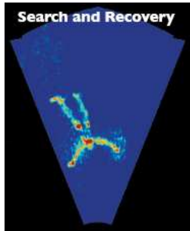
In this sonar image, the body of a swimmer is clearly visible. Once detected, the operator can then use the sonar to monitor and direct recovery operations.
