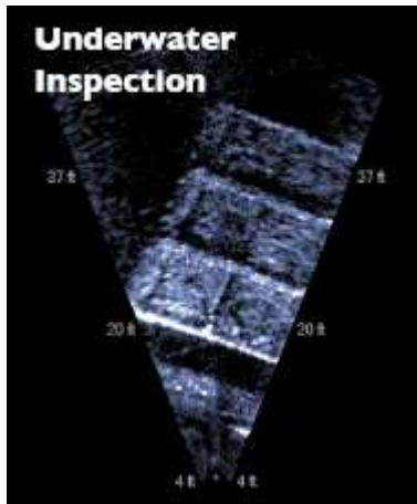
This image shows the bottom side of a floating dock at close range. The dock's structure and features are clearly visible in even the murkiest conditions.
