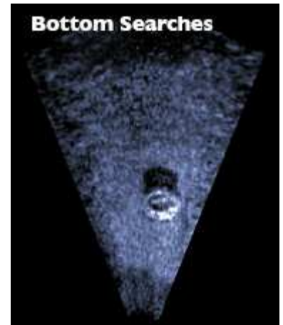
Quickly locate and navigate to objects, even in low visibility conditions. The above sonar image shows a tire located during an ROV-based search operation.
